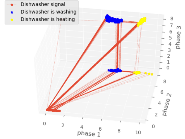
Fig. 8: Dishwasher signal trajectory in a 3-dimensional PP with phases 1, 2, and 3 as the coordinate axes
