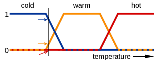
Fig. 2: Illustration describing the level of temperature with fuzzy logic
