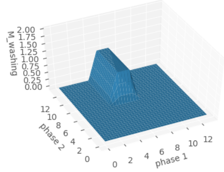
(a) Output membership function for washing: \mathcal{M}_{\text{washing}}(p_1, p_2)
