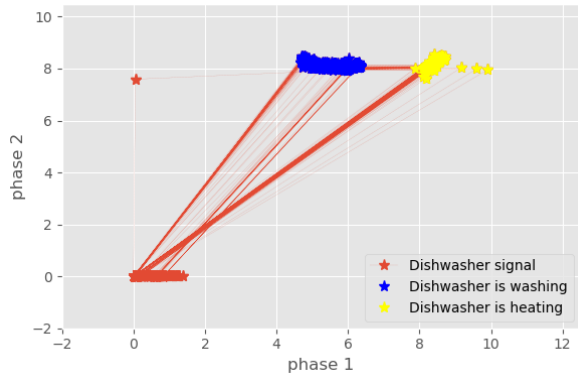
Fig. 7: Dishwasher signal trajectory in a 2-dimensional PP with phase 1 and phase 2 as the coordinate axes
