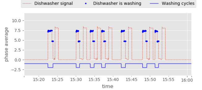
Fig. 15: Dishwasher phase average signal with labelled washing operation and washing cycles (lower value on the line indicate the washing cycles)
