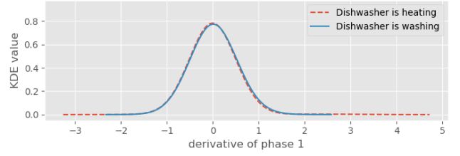
(a) KDE for the washing & heating operations on \dot{p}_1
