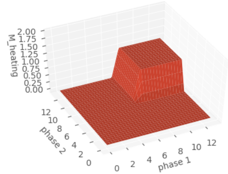
(b) Output membership function for heating: \mathcal{M}_{\text{heating}}(p_1, p_2)
