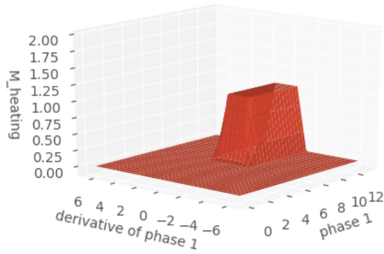
(b) Membership function for heating: \mathcal{M}_{\text{heating}}(p_1, \dot{p}_1)
