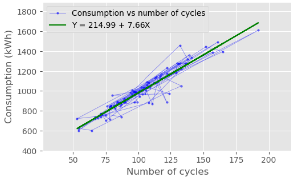
Fig. 17: Correlation and regression model between dishwasher daily energy consumption and number of washing cycles, during the period July 2019 to September 2019
