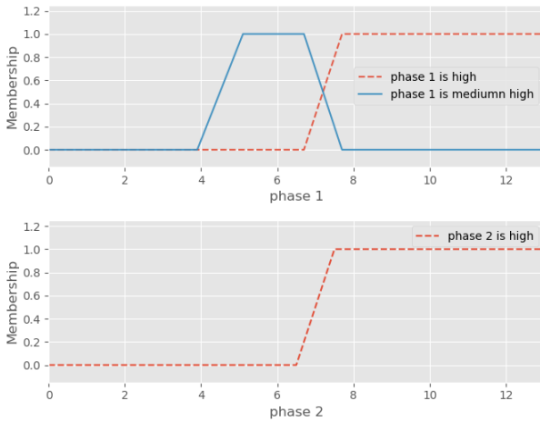
Fig. 10: Membership functions for fuzzy sets \mathcal{M}_{1h}(p_1) , \mathcal{M}_{1mh}(p_1) and \mathcal{M}_{2h}(p_2)
