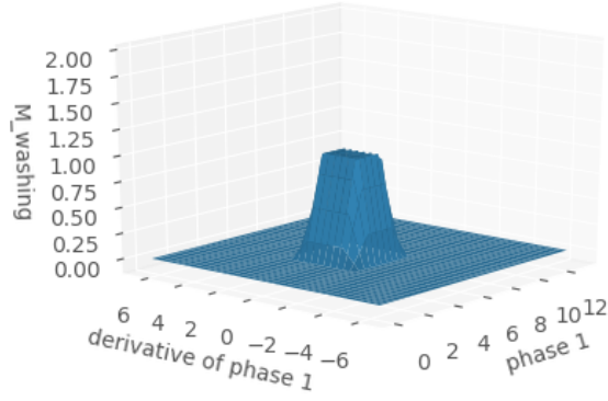
(a) Membership function for washing: \mathcal{M}_{\text{washing}}(p_1, \dot{p}_1)
