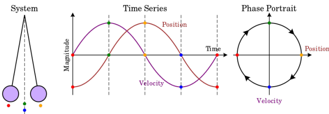
Fig. 1: Illustration of how a phase portrait would be constructed for the motion of a simple pendulum.
