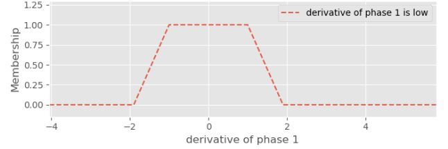
(b) Membership function for \mathcal{M}_{d1l}(\dot{p}_1)
