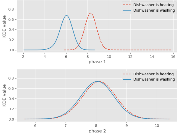
Fig. 9: Kernel density estimation for the washing and heating operations on phase 1 and phase 2
