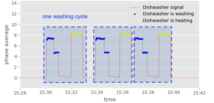
Fig. 5: Dishwasher signal with labelled heating and washing operation fractions
