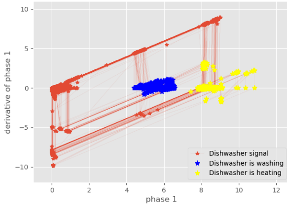
Fig. 12: Dishwasher signal trajectory in a 2-dimensional PP with phase 1 and its derivative as the coordinate axes
