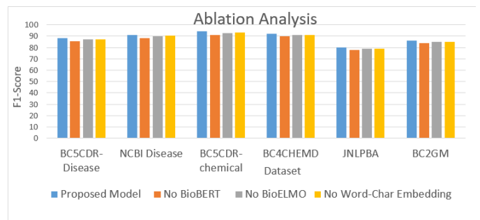
Fig. 2. Ablation Analysis of proposed model.
