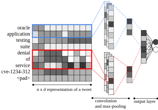
Fig. 2. Convolutional neural network architecture for sentence classification.
