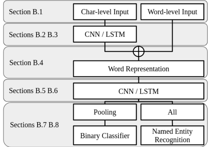
Fig. 5. Multi-Task Learning model architecture.
