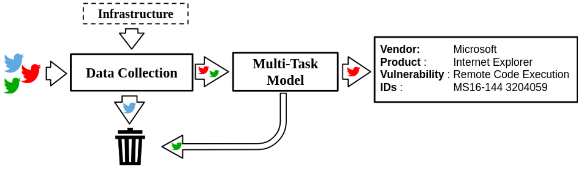
Fig. 4. MTL-based cyberthreat intelligence pipeline.
