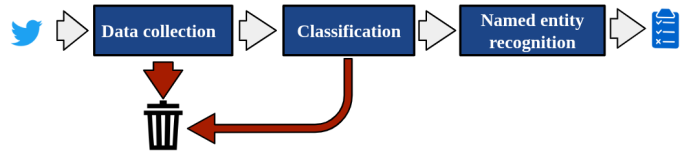
Fig. 1. Previous work Twitter-based threat detection pipeline architecture with single-task DNN [5].
