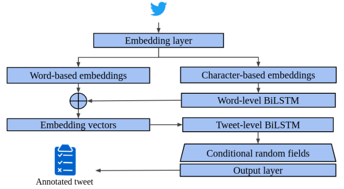
Fig. 3. Bidirectional long short-term memory architecture for named entity recognition.
