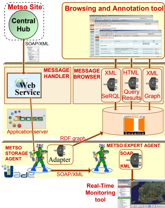
Figure 5: Agent-enabled system.
