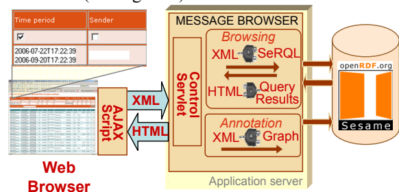
Figure 4: Client-server interaction.
