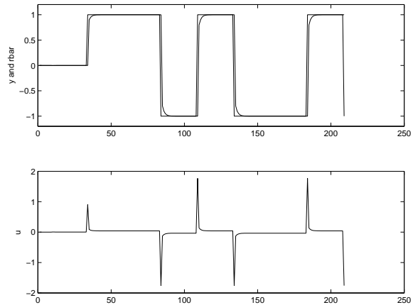
Figure 5: Performance with a linear model.
