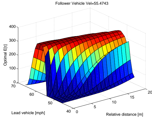
Fig. 4. A cross-section of approximate optimal value function.
