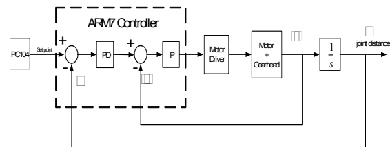
Figure 5: Joint controller.
