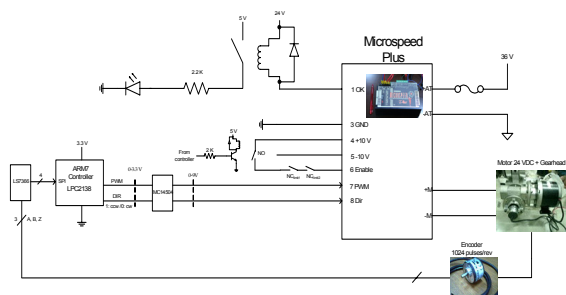
Figure 6: Servo interfacing circuit.
