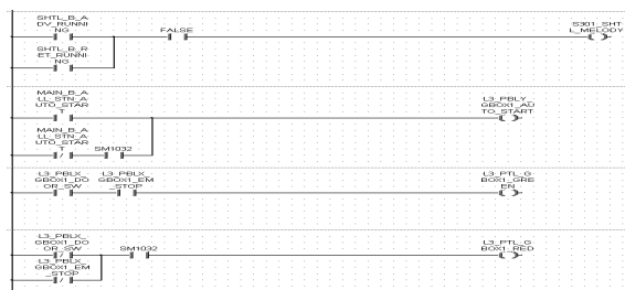
Figure 1: The PLC code in the form of Ladder diagram.
