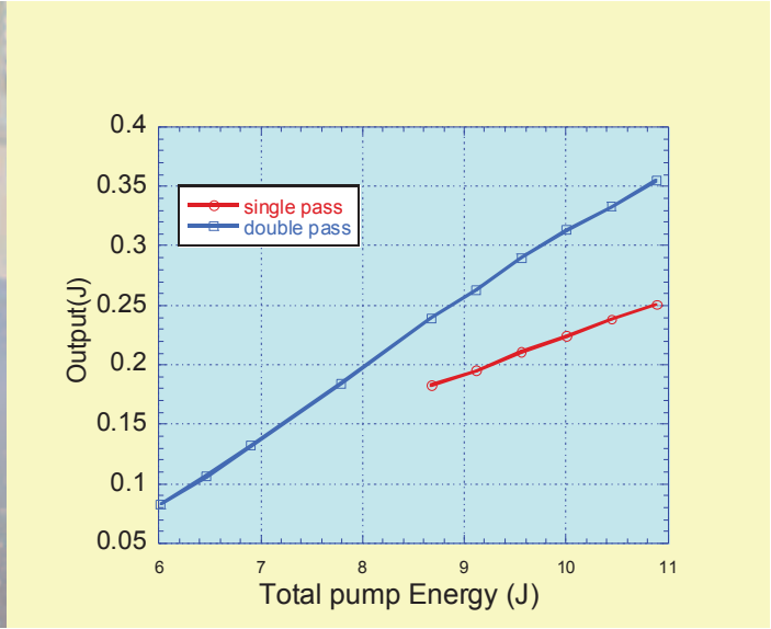
Fig 2. Amplifier performance with 100mJ input from the oscillator
