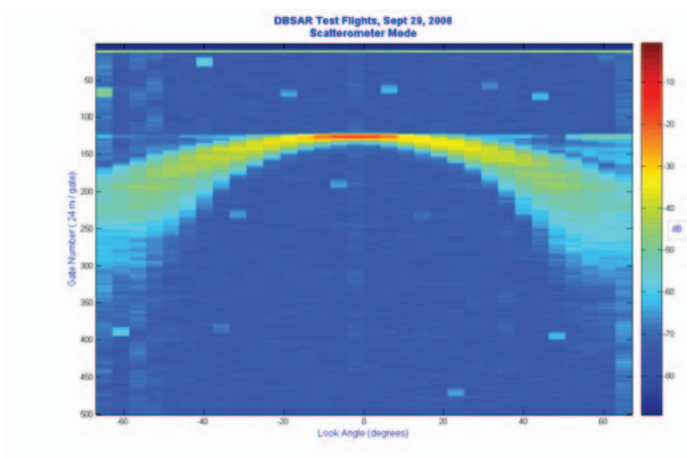
Figure 1 Plot of DBSAR's scatterometer mode showing backscatter power vs. look angle for a scan range from -65 to +65 degrees.
