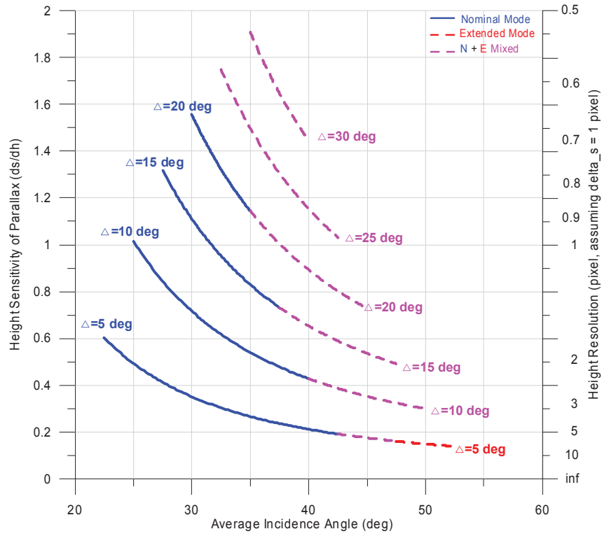
Fig. 1. The height sensitivity of parallax and the height resolution of KOMPSAT-5 as a function of the average incidence angle. The delta is the difference of incidence angle between the radargrammetric image pair [4].
