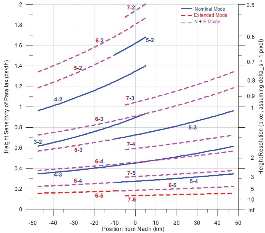
Fig. 2. The height sensitivity of parallax and the height resolution of radargrammetric image pairs of KOMPSAT-5 as a function of the position from nadir. A pair of pass numbers is given on each line [4].
