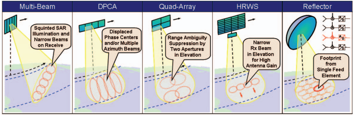
Figure 2– Solutions for high-resolution wide-swath SAR imaging. Left: multiple beam SAR. Middle left: displaced phase center antenna technique. Middle: quad-element rectangular array SAR. Middle right: high-resolution wide-swath (HRWS) SAR. Right: High resolution wide swath SAR employing a reflector antenna in combination with a digital feed array.
