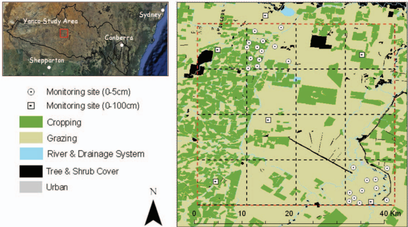
Fig. 1: Location and land use conditions in the SMAPEX Yanco study area, corresponding to the SMAP 36km x 36km grid (red rectangle), and the ground sampling focus areas corresponding to the SMAP 9km x 9km grid (black rectangles). Locations of the continuous monitoring stations are indicated with white circles and squares.
