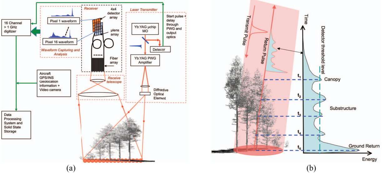
Figure 1. (a) IIP airborne instrument concept; (b) interpretation of time-of-flight information on the return pulse into vegetation heights and ground return.
