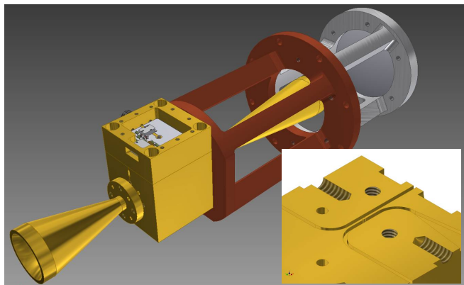
Fig. 3. 3D assembling model of the sis mixer block with diagonal feed horn
