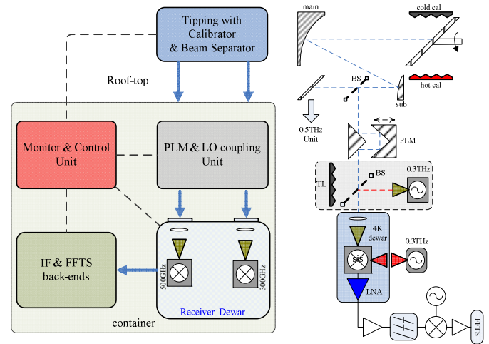
Fig. 2. The radiometer system (left) and its lower band details (right)
