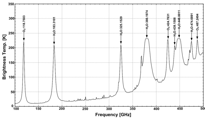
Fig. 1. Simulated atmosphere spectra (Tibet winter season) with AM 7.0[4]
