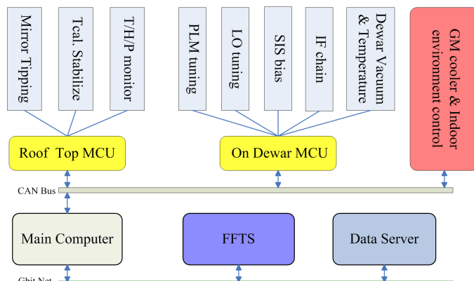
Fig. 4. The overall control and data acquisition system for the dual-band THz radiometer.
