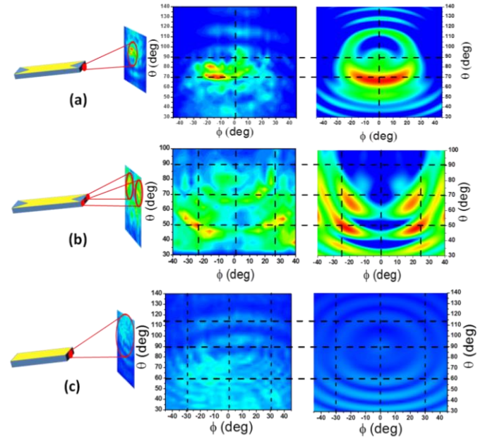
Fig. 1. Simulated far-field patterns (right side) of metal-metal THz QCLs and their corresponding far-field patterns measured at 77K (left). (a) 40µm-wide metal-metal THz QCL (b) 80µm-wide metal-metal THz QCL. (a) and (b) are with ~150µm-long planar horn antennas integrated onto QCL top metal at both side of the facet. (c) 60µm-wide metal-metal THz QCL without any planar horn antenna.
